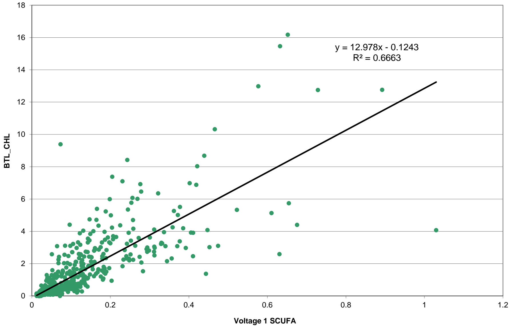
CalCOFI 0504NH: SCUFA Fluorometer Voltage 1 vs Bottle Chl-a 4sec ave voltage vs bottle chl-a (mg/m 3 )
