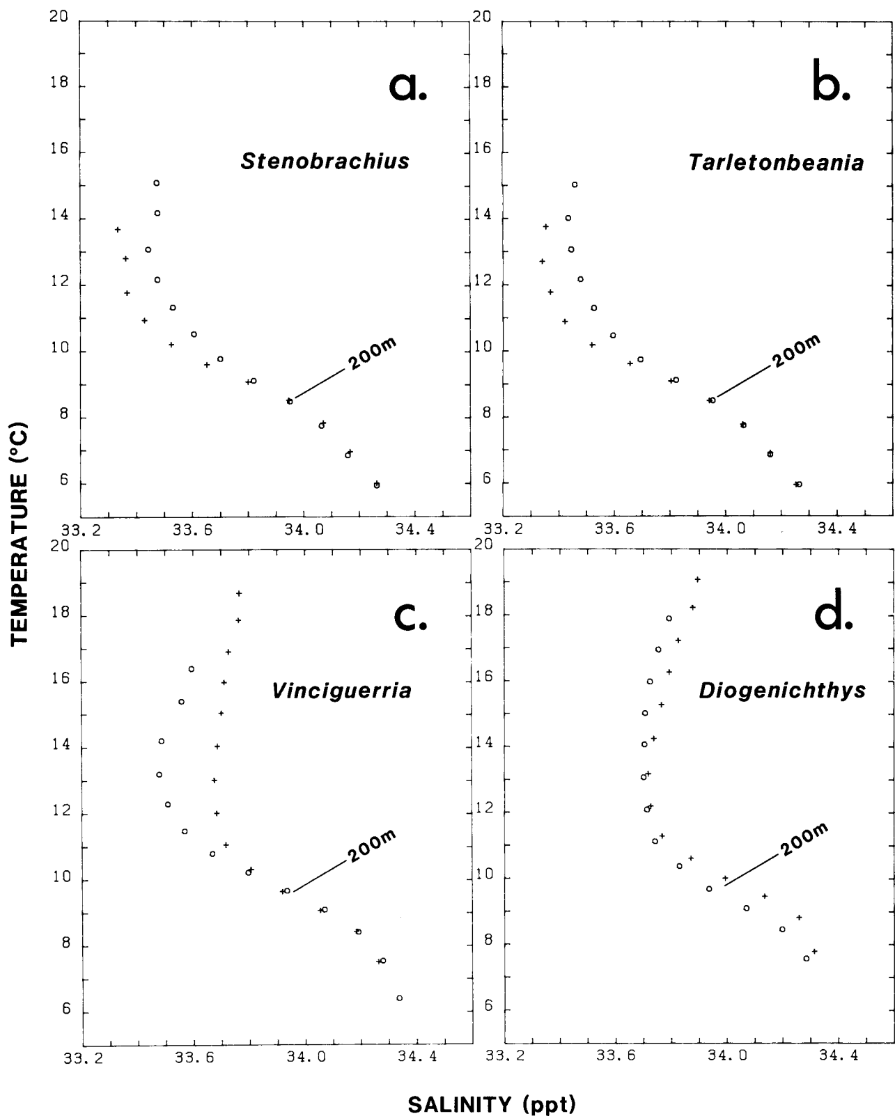
Figure 11. a. Mean temperature-salinity curves depicting differences in watermass characteristics associated with the absence (o) or presence (+) of Stenobranchius leucopsarus larvae in CalCOFI net tows. The plots represent combined data from 16 offshore stations on lines 83-100 (see Figure 1) occupied during 1954-60. b. Same as a for Tarletonbeania crenularis larvae. The data represented in the figure are from 14 offshore stations on lines 83-100. c. Same as a, for Vinciguerria lucetia larvae. The data represented in this figure are from 21 offshore stations on lines 100-120. d. Same as a, for Diogenichthys laternatus larvae. The data represented in this figure are from 17 offshore stations on lines 103-120.
