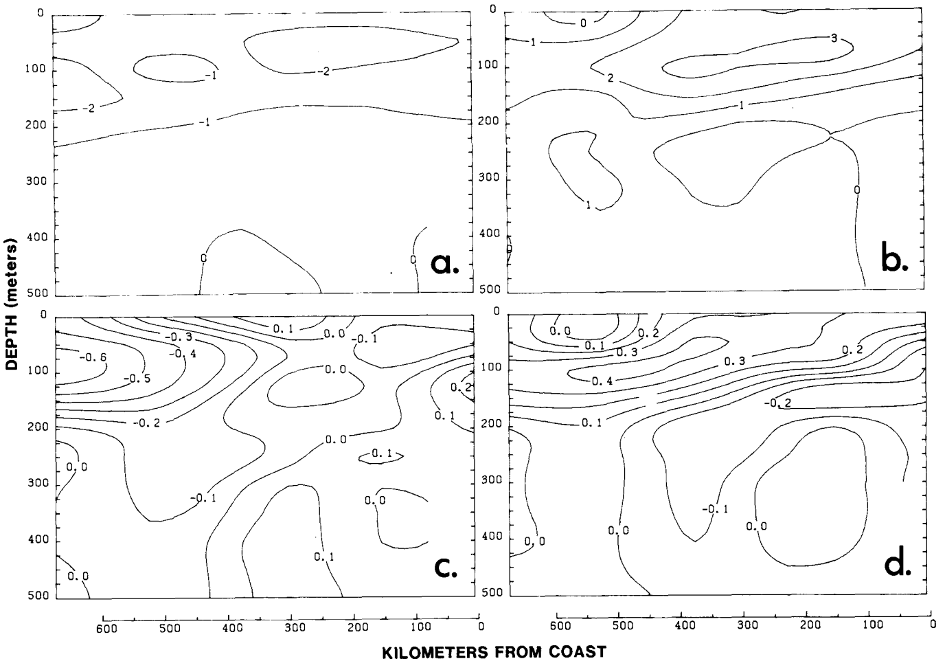
Figure 5. Mean temperature anomaly pattern along CalCOFI line 100 in the upper 500 meters, 1955-56 (a), and 1958-59 (b). Mean salinity anomaly pattern (computed in the same way) for 1955-56 (c) and 1958-59 (d). The isopleths represent deviations from harmonic means based on the period 1950-78.
