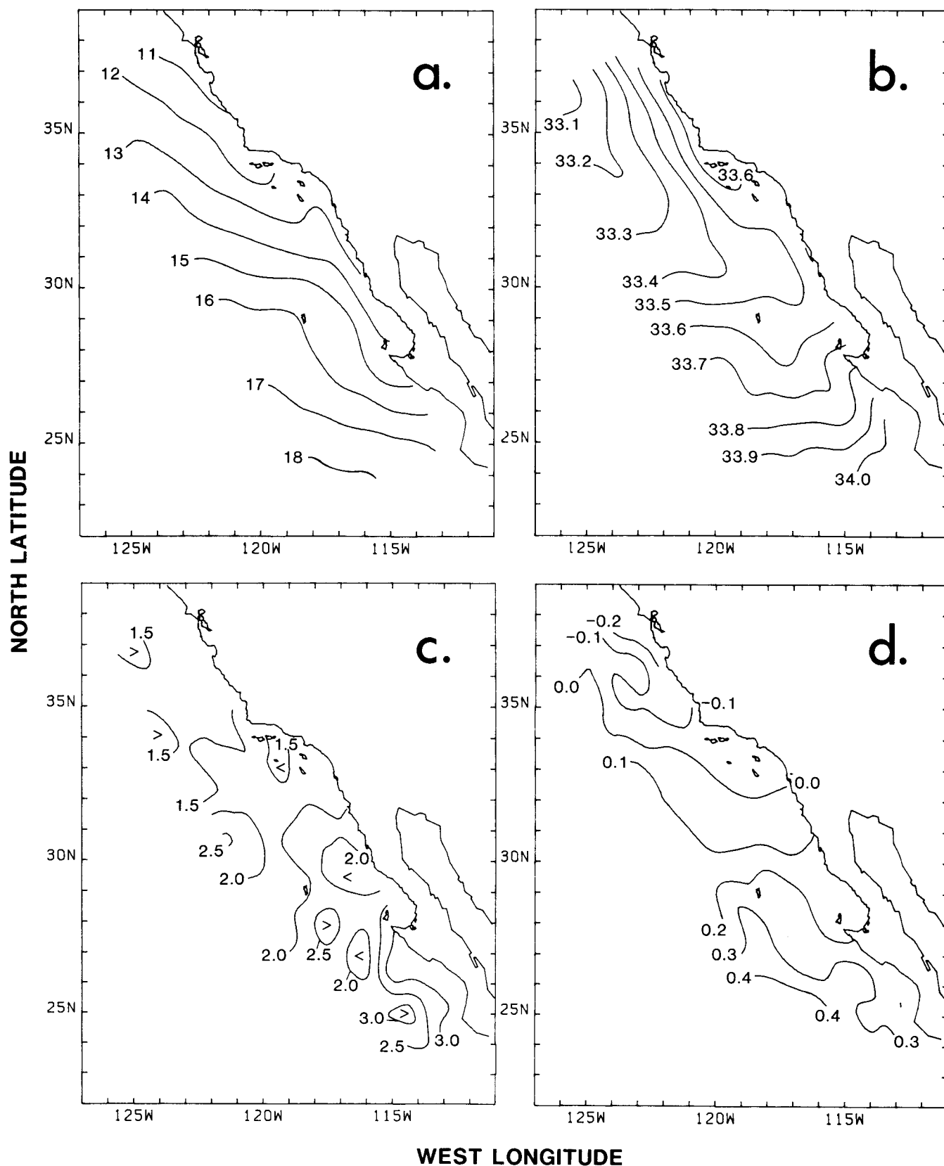
Figure 3. Mean annual temperature (a) and salinity (b) of the upper 100 meters computed at 5 standard depths (10 m, 30 m, 50 m, 75 m, and 100 m) from harmonic coefficients based on data from CalCOFI cruises from 1950 through 1978. Change, or difference, in the deviations of temperatures (c) and salinities (d) in the upper 100 meters from the harmonic means, between the periods 1955-56 and 1958-59.
