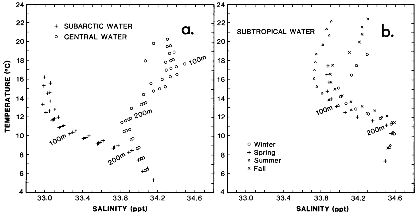
Figure 2. Mean seasonal temperature-salinity plots for modified subarctic water and Pacific central water (a) and subtropical water (b) in the California Current region. The symbols are plotted for discrete values of sigma-t at intervals of 0.2 g/l.
