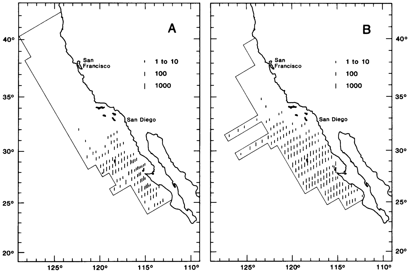
Figure 2. Change in distribution of larvae of Vinciguerria lucetia during cold (A) and warm (B) temperature regimes in the California Current region. Pooled numbers of larvae for three cold years (1954–56) and three warm years (1958–60) are indicated by exponentially scaled bars. The survey pattern for each series of years is outlined.
