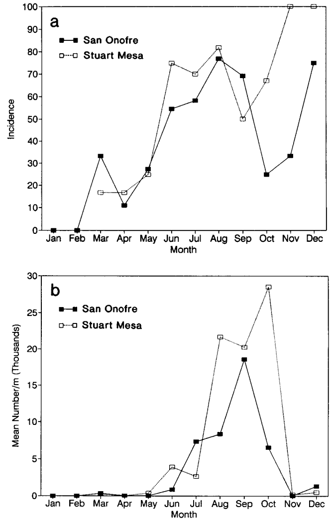
Figure 6. a, Monthly mean incidence (percent positive collections) and b, abundance (number under a 1-m-wide strip between the 6-m and 75-m isobaths) of larval Pacific sardine. All developmental stages and all years are pooled.
