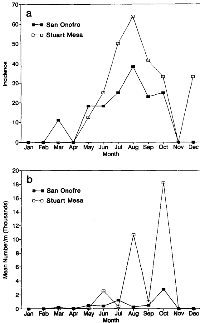
Figure 8. a, Monthly mean incidence (percent positive collections) and b, abundance (number under a 1-m-wide strip between the 6-m and 75-m isobaths) of yolk-sac larval Pacific sardine. All years are pooled.
