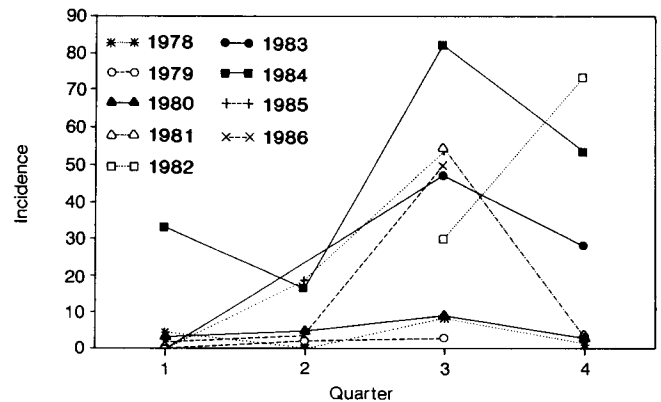
Figure 7. Incidence (percent positive collections) of larval Pacific sardine, 1978-86, plotted by quarter. All developmental stages, and data from both study sites are pooled.
