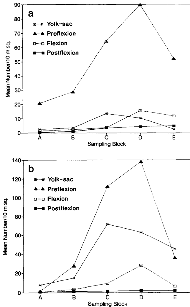
Figure 3. Mean number of larval Pacific sardine under 10 m 2 of sea surface in each sampling block. Each developmental stage is plotted separately; all years are pooled. a = San Onofre; b = Stuart Mesa.
