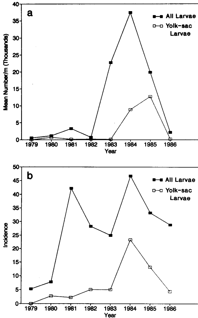
Figure 10. a, Annual mean abundance (number under a 1-m-wide strip between the 6-m and 75-m isobaths) and b, incidence (percent positive collections) of larval Pacific sardine off Stuart Mesa.
