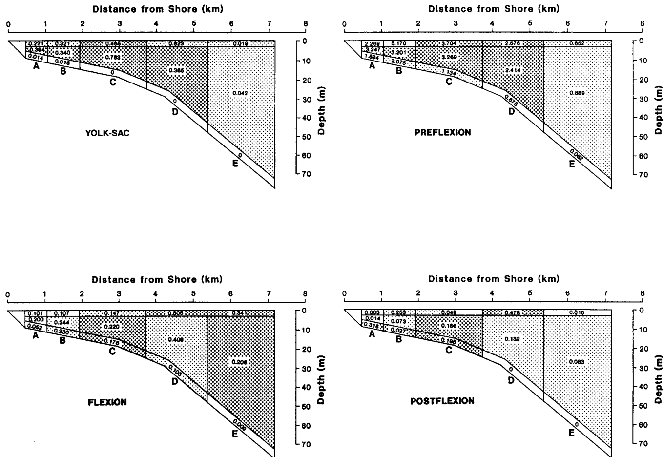
Figure 4. Mean number of larval Pacific sardine per 100 m 3 of water in each stratum (neuston, midwater, epibenthos) in each sampling block at San Onofre. Each developmental stage is plotted separately; all years are pooled. Neustonic and epibenthic strata are vertically exaggerated in these schematic representations. Shading indicates rankings of the geometric mean densities from the ANOVA on density: dark = the five highest-ranked means; light = the five middle-ranked means; white = the five lowest-ranked means.
