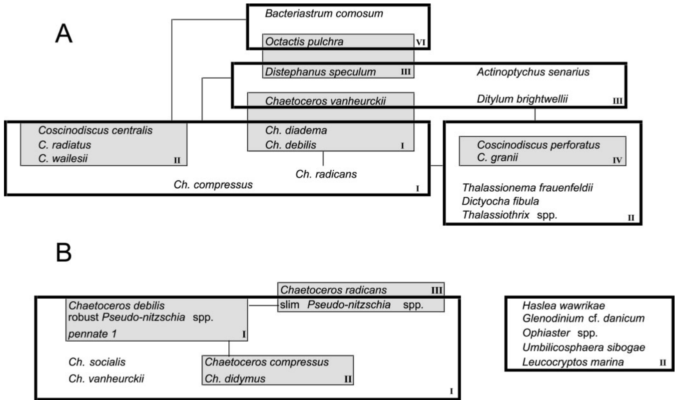
Figure 7. Recurrent groups of species defined at \alpha = 0.70 (shaded boxes) and at \alpha = 0.55 (unshaded boxes): A, trap samples; B, water samples. Composition of a recurrent group is indicated within a box. Lines between boxes (or between a species and a box) indicate association between groups or between a species and a group. Thus, in the trap samples, the species of group II and IV at \alpha = 0.70 continue to be associated at \alpha = 0.55 . Groups I and III at \alpha = 0.70 are each split into two groups at \alpha = 0.55 . Not all groups at \alpha = 0.55 are shown.
