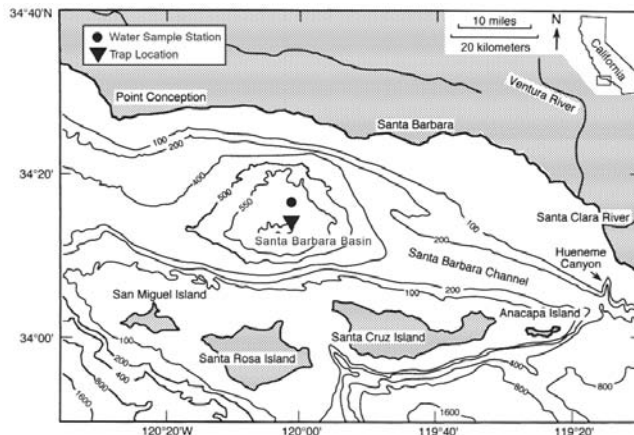
Figure 1. Geographic and topographic map of the Santa Barbara Channel and the Santa Barbara Basin showing the locations of the sediment trap and the water sample station.
