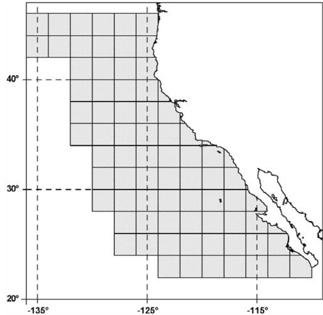
Figure 1. The COADS quadrants used to obtain the annually averaged sea-surface temperature anomalies for the California Current system.
