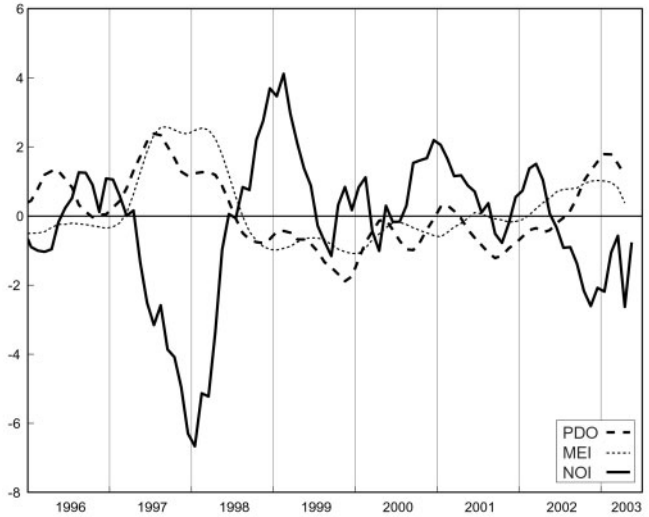
Figure 3. Monthly time series of the Pacific Decadal Oscillation (PDO), Multivariate ENSO Index (MEI), and Northern Oscillation index (NOI) for January 1996 through April (May) 2003 for PDO and MEI (NOI). Series have been smoothed with a 5-month running mean, except the last two months, which are raw values.
