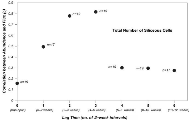
Figure 4. Correlation between abundance and flux of total siliceous phytoplankton at lag times from zero to six 2-week intervals, with abundance leading flux.
