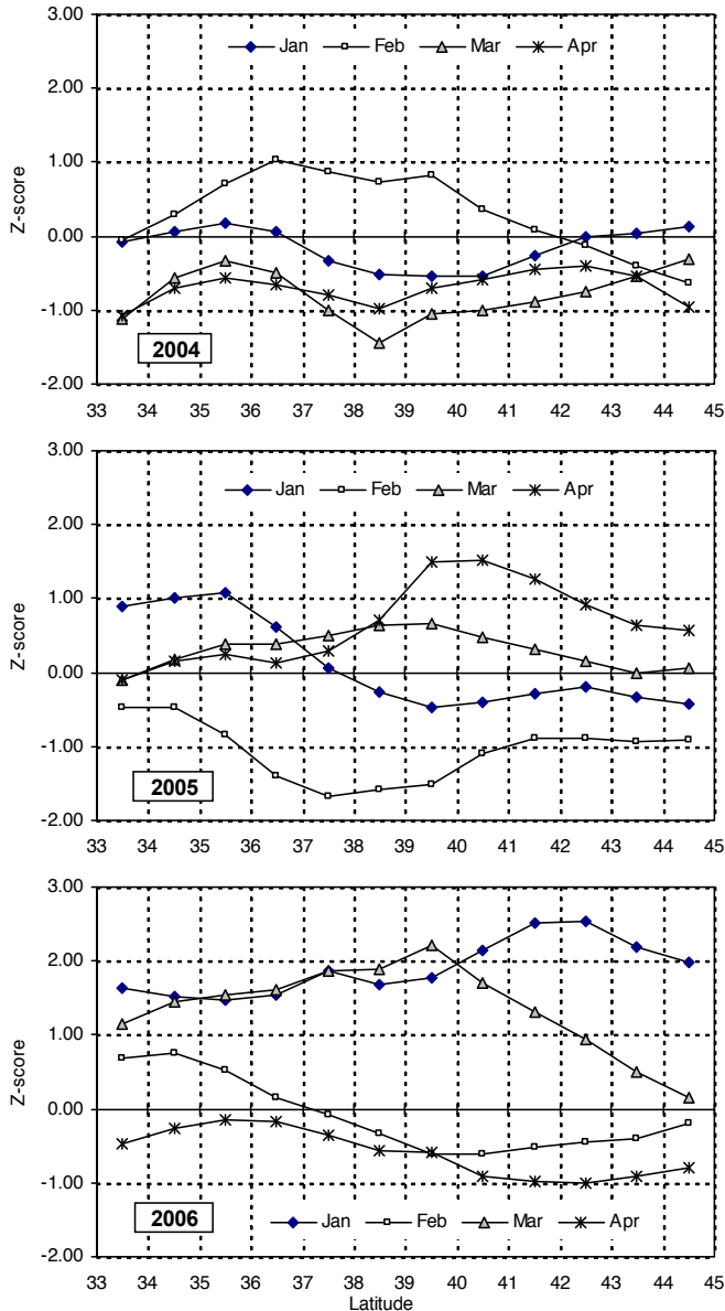
Figure 6. Seasonal and spatial variability in zonal wind stress from 2004–06 relative to the climatology. Z-scores are calculated as standardized deviations from the long-term mean ( \mu ) and standard deviation ( \sigma ) (see text for further explanation).
