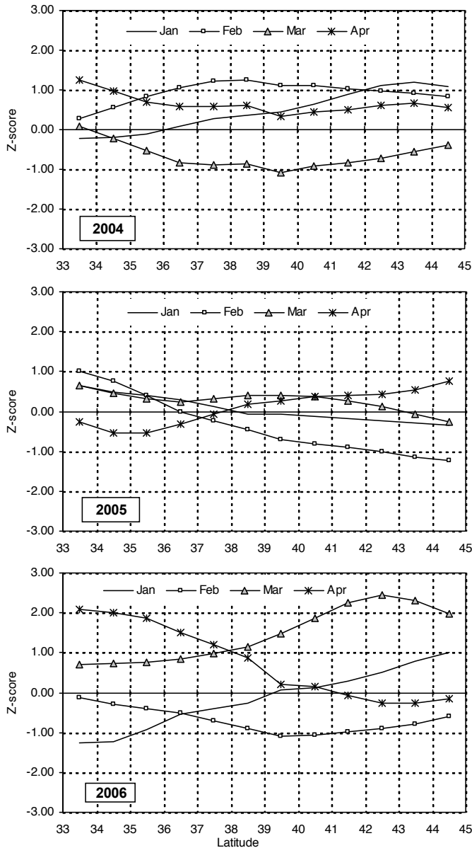
Figure 7. Seasonal and spatial variability in meridional wind stress from 2004–06 relative to the climatology. Z-scores are calculated as standardized deviations from the long-term mean ( \mu ) and standard deviation ( \sigma ) (see text for further explanation).
