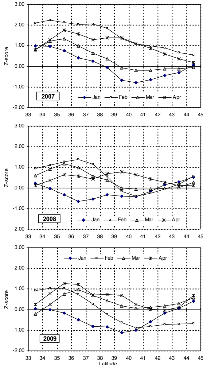
Figure 6 (cont'd). Seasonal and spatial variability in zonal wind stress from 2007–09 relative to the climatology.
