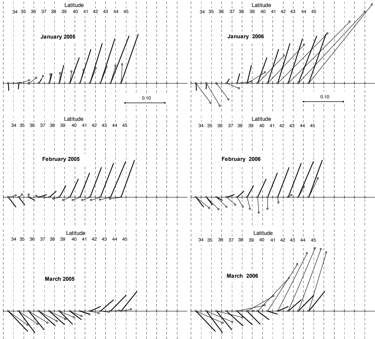
Figure 8. Latitudinal distributions of January–March wind stress vectors during 2005 and 2006 (fine lines with small open squares). Expected wind stress vectors based on climatological means are shown as bolded lines.
