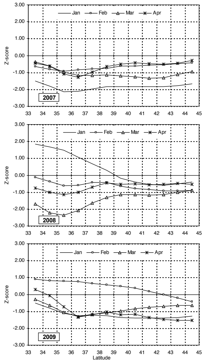
Figure 7 (cont'd). Seasonal and spatial variability in meridional wind stress from 2007–06 relative to the climatology.
