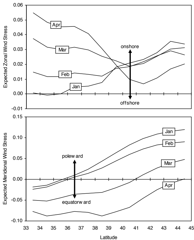
Figure 5. Climatology of wind stresses on the U.S. West Coast in the months preceding the midwater trawl survey (January–April). The upper panel shows zonal (east-west) winds and the lower panel depicts meridional (north-south) winds. Expected wind stresses are based on average values calculated over the period 1970–2011.
