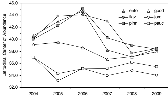
Figure 4. Time series of the average latitudes of survey catches for commonly-sampled juvenile rockfishes taken in the SWFSC-NWFSC midwater trawl survey (legend = first four letters of scientific name).
