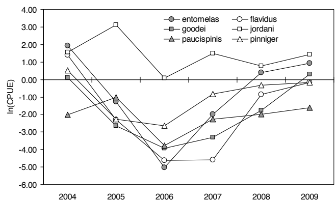
Figure 2. Annual trends in catch-per-unit-effort (CPUE) of pelagic juvenile rockfishes collected in the midwater trawl survey.
