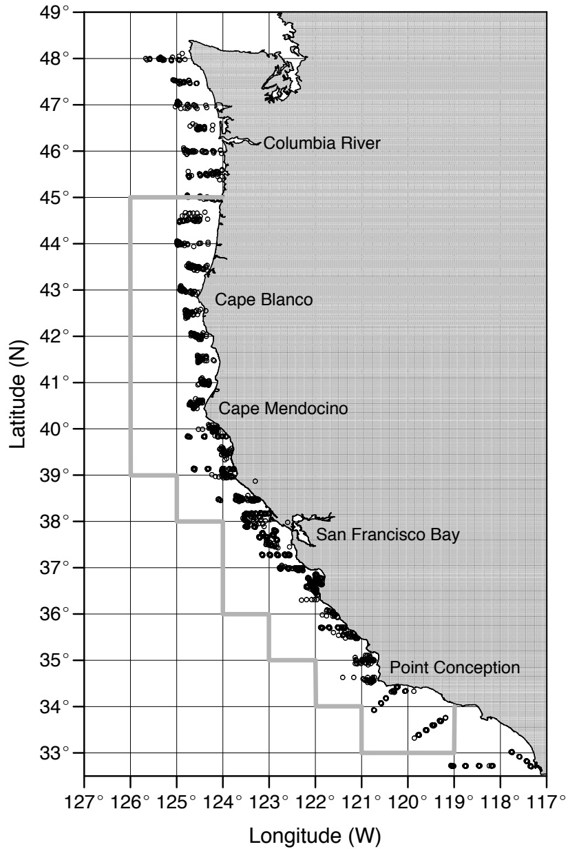
Figure 1. Map of the U.S. West Coast showing the spatial extent of the combined SWFSC-NWFSC pelagic juvenile rockfish midwater trawl survey (2001–09). Trawl sampling stations shown as small open circles; wind stress calculations based on 1° x 1° latitude-longitude cells occurring within the bold gray polygon.
