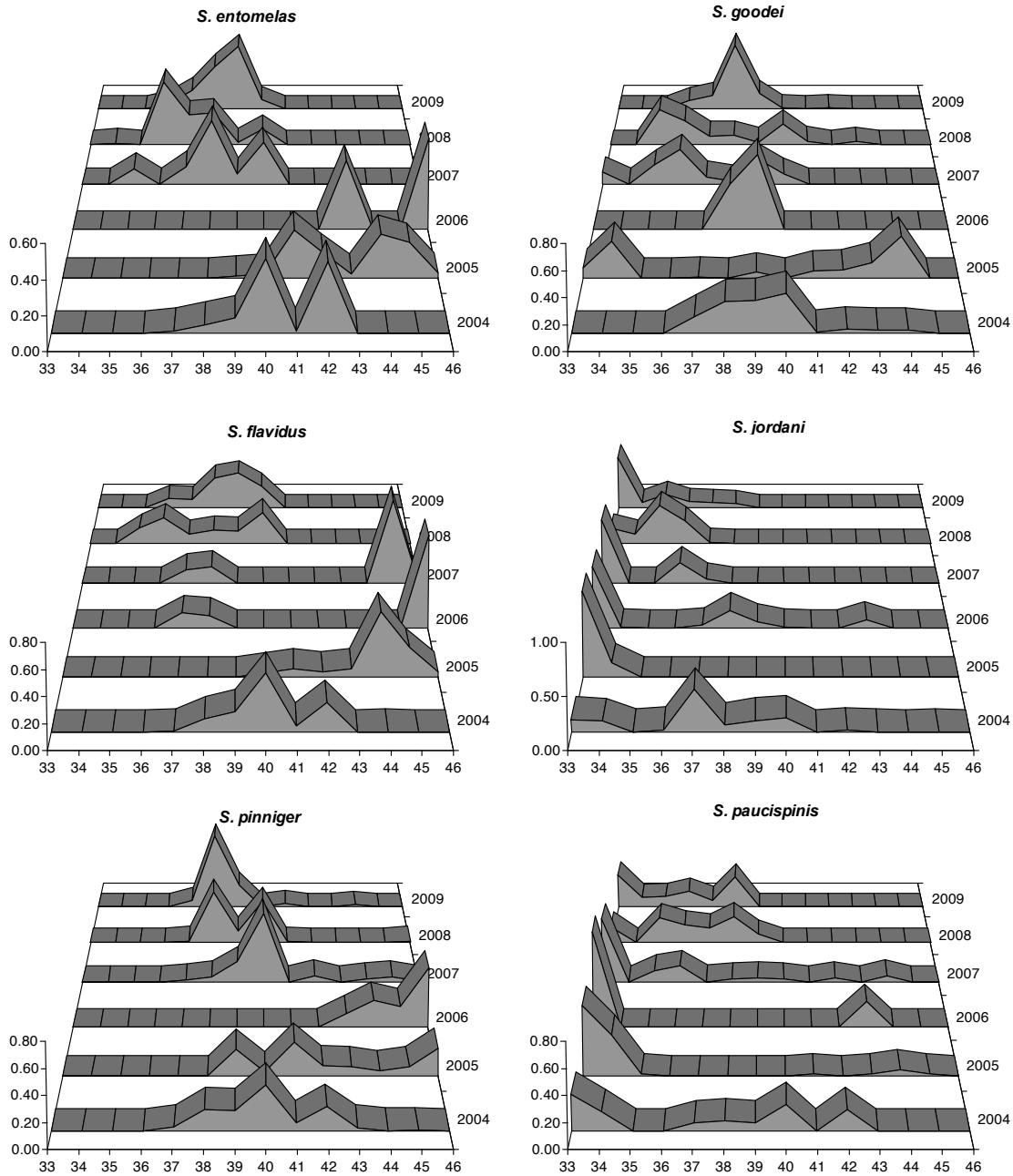
Figure 3. Spatial distributions of normalized CPUE for 6 Sebastes spp. from 2004–09. Plotted on the x-axis is latitude, on the y-axis is year, and on the z-axis is the proportion of spatially integrated annual CPUE.
