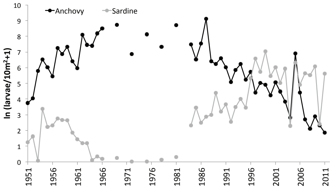
Figure 29. Abundance ( \ln(\text{number}/10\text{m}^2+1) ) of northern anchovy and Pacific sardines captured in oblique tows (bongo net) during spring CalCOFI surveys 1951–2011.
