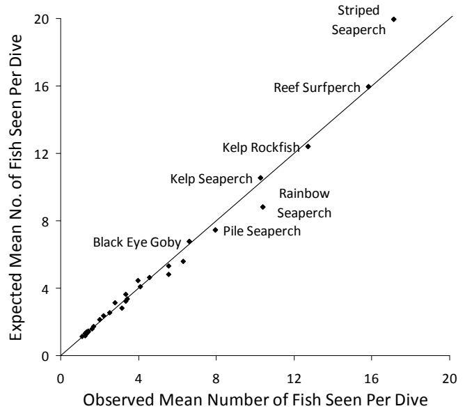
Figure 6: Model 3's expected versus observed mean number of fish sighted per dive for various species (each data point represents an observed fish species). Data from a perfect predictive model would fall on a 1:1 line. Figure 6a (left graph) shows the full range of species' predicted and observed counts (0–160). Figure 6b (right graph) shows that most species cluster in the region of 20 or fewer average sightings per dive.
