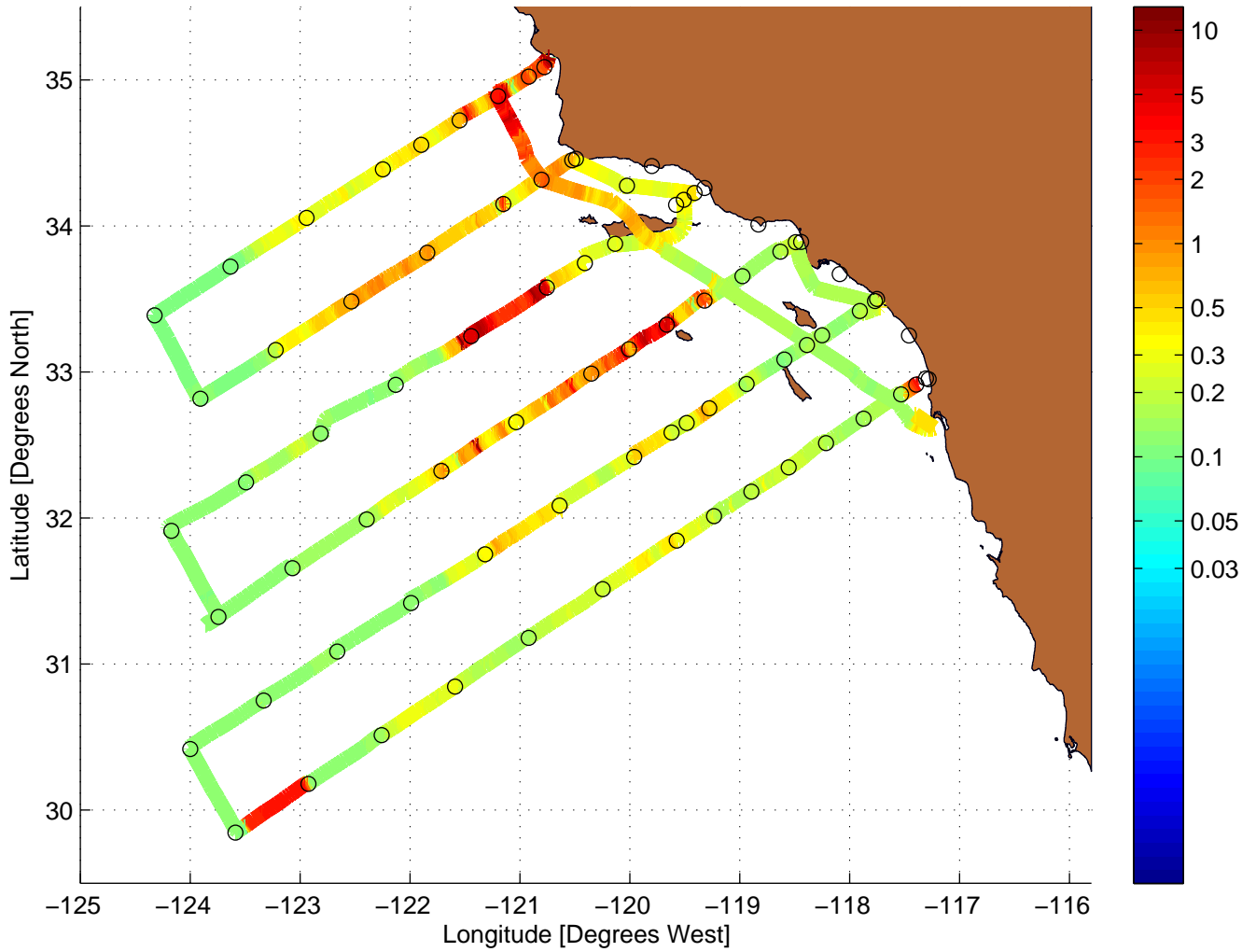
Chlorophylla Value Along CalCOFI Cruise: 9707NH
