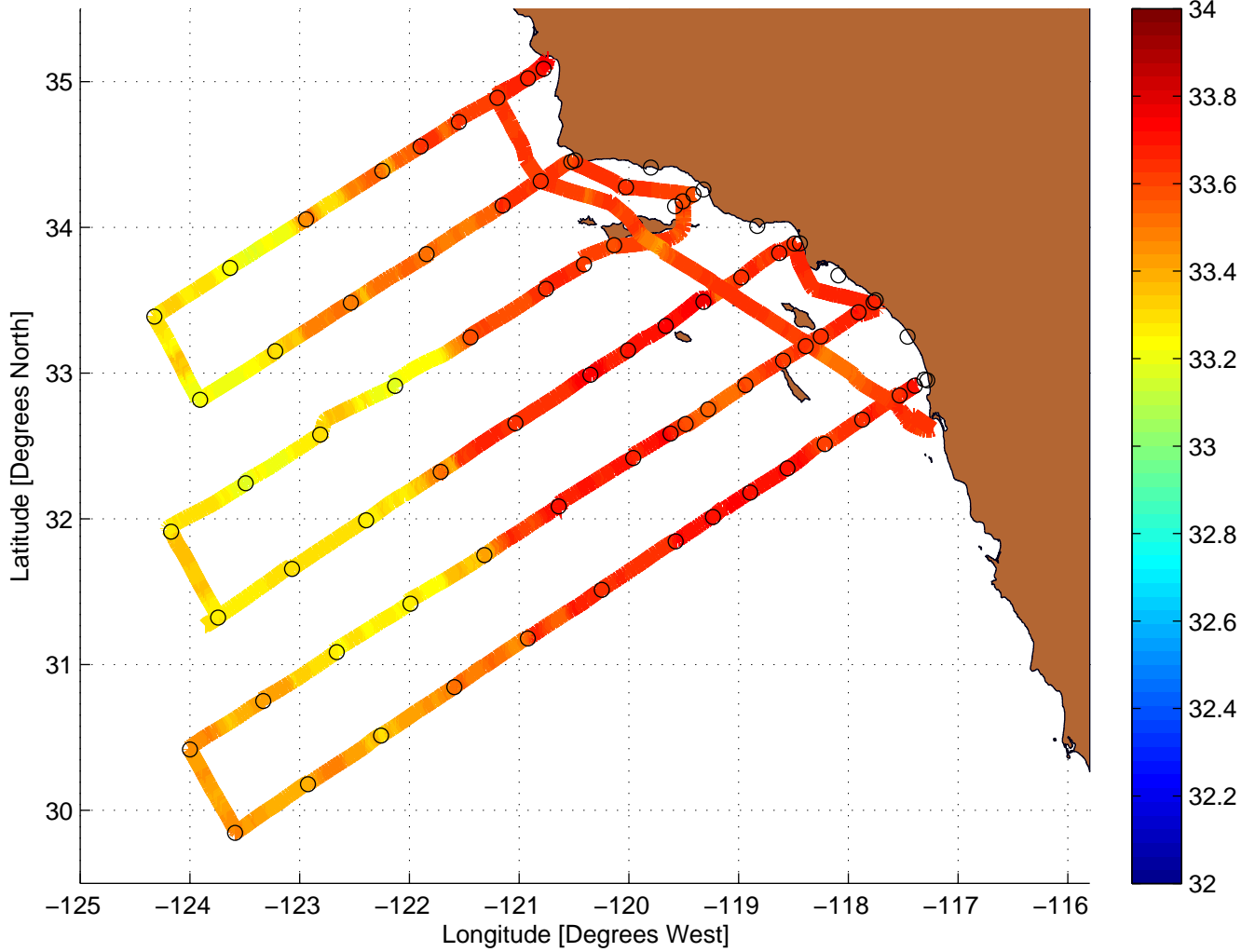
Salinity Value Along CalCOFI Cruise: 9707NH
