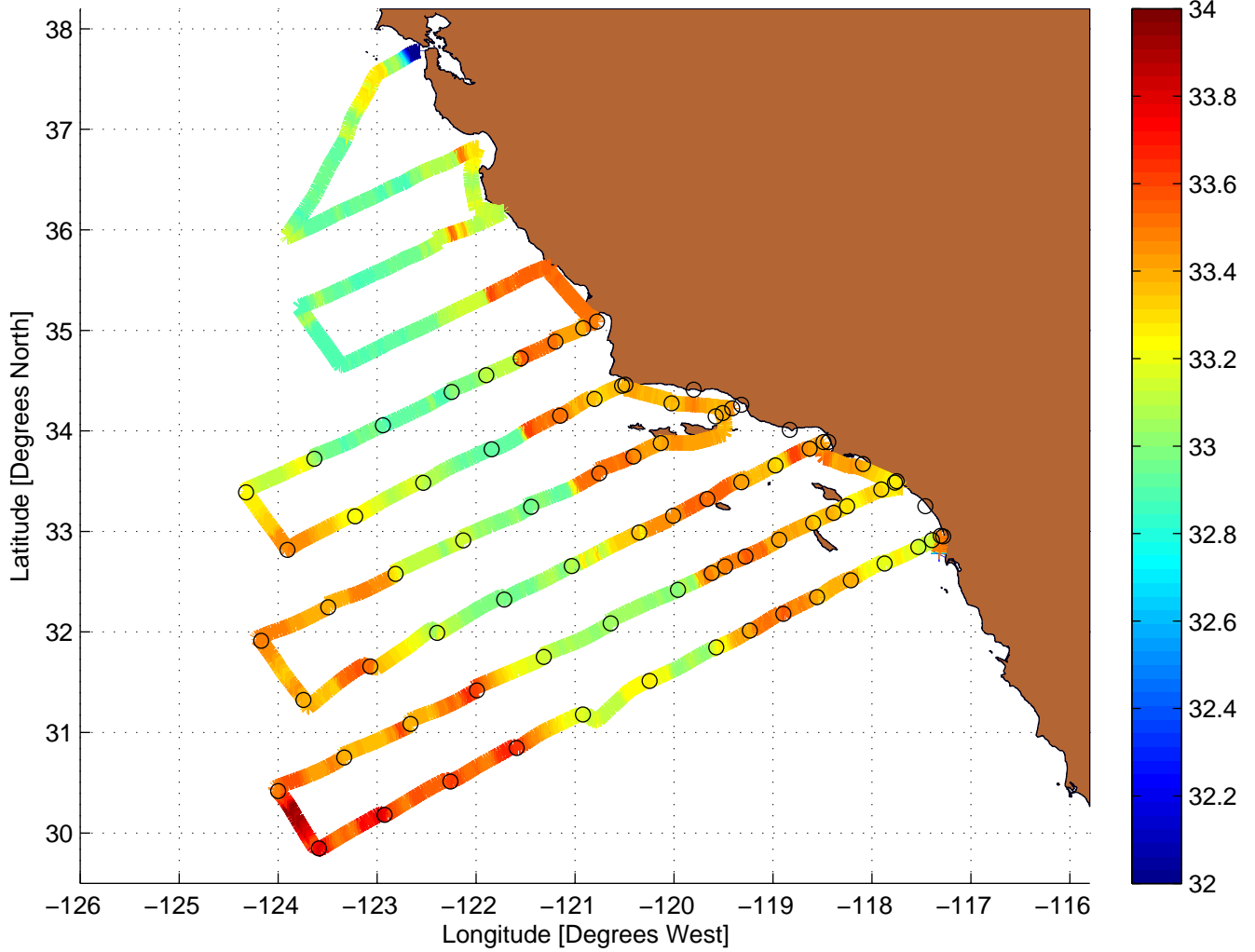
Salinity Value Along CalCOFI Cruise: 9807NH
