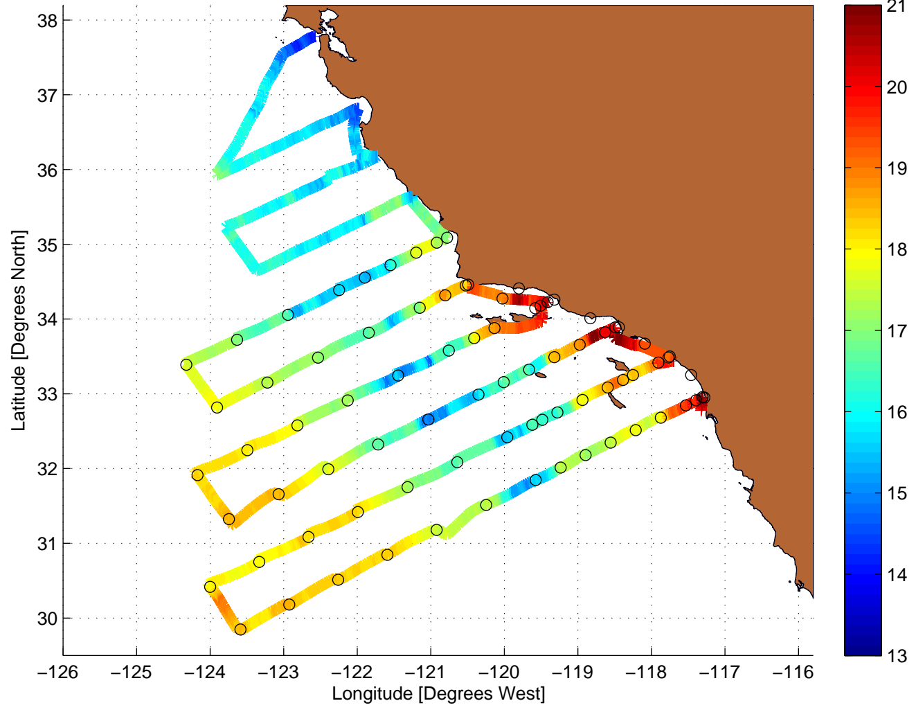
Temperature Value Along CalCOFI Cruise: 9807NH
