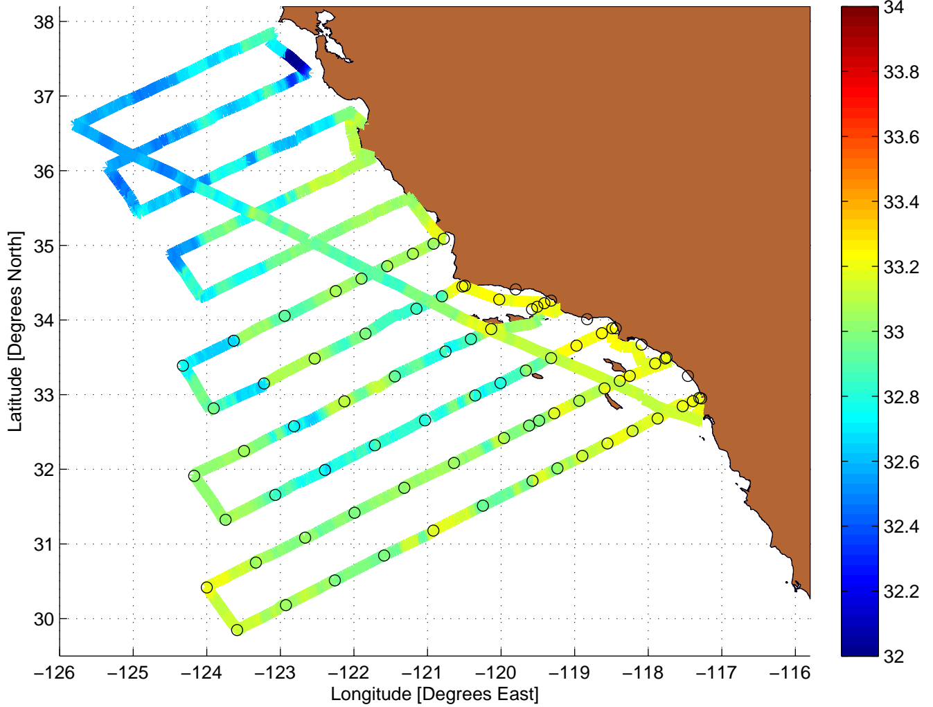
Salinity Value Along CalCOFI Cruise: 0401JD
