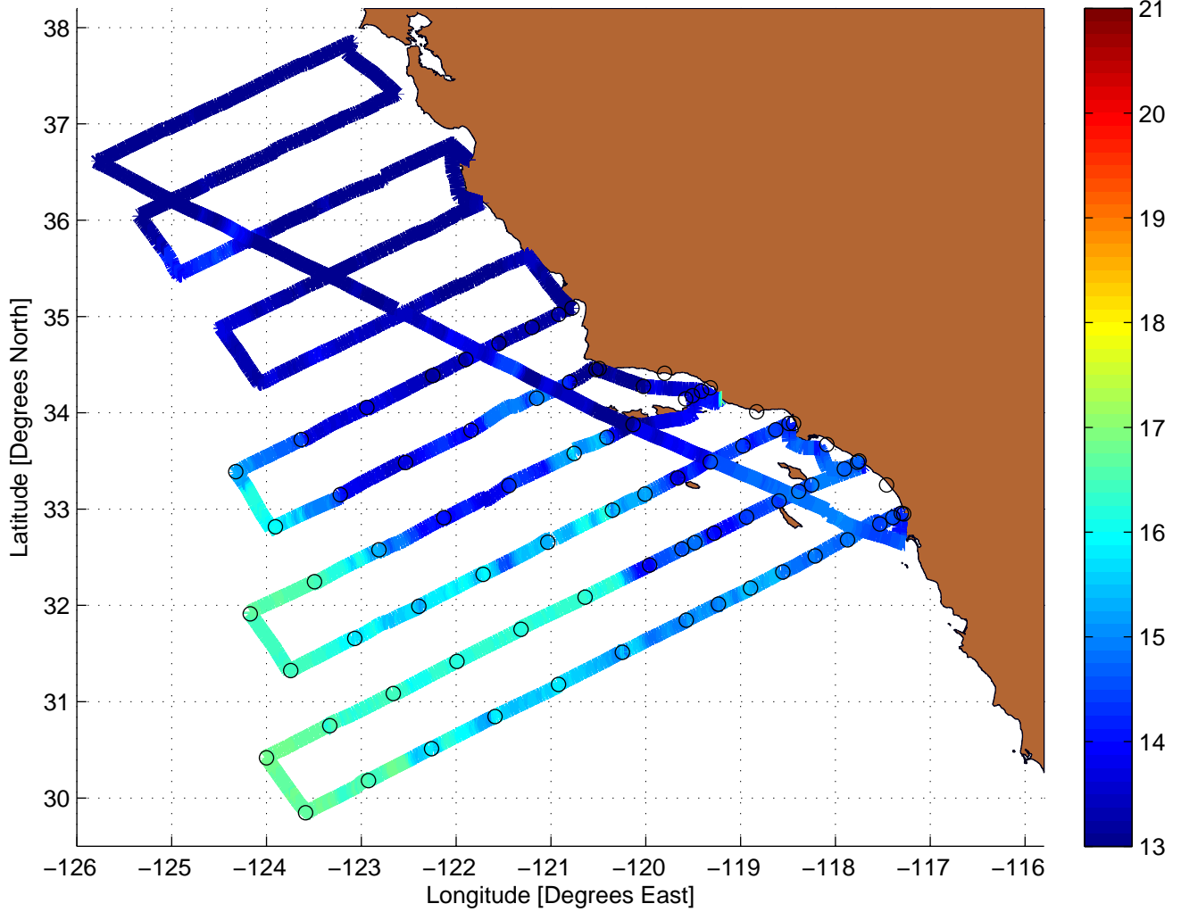
Temperature Value Along CalCOFI Cruise: 0401JD
