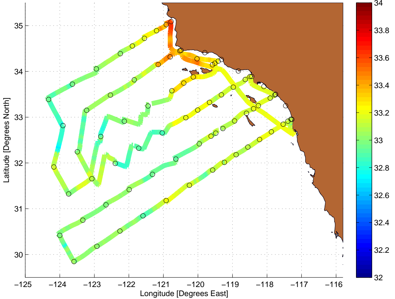
Salinity Value Along CalCOFI Cruise: 0404NH
