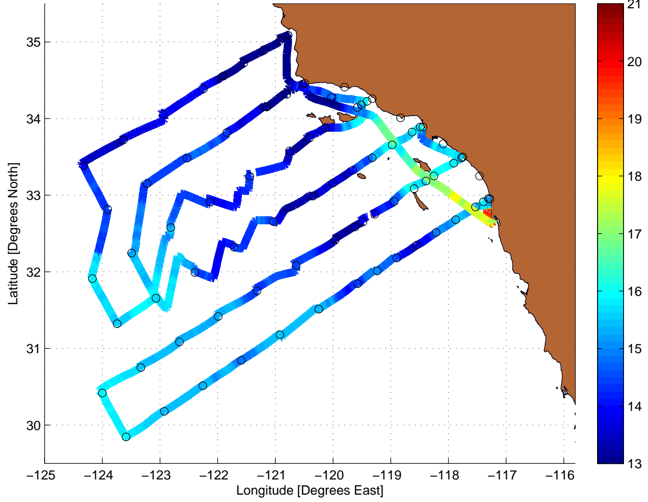
Temperature Value Along CalCOFI Cruise: 0404NH
