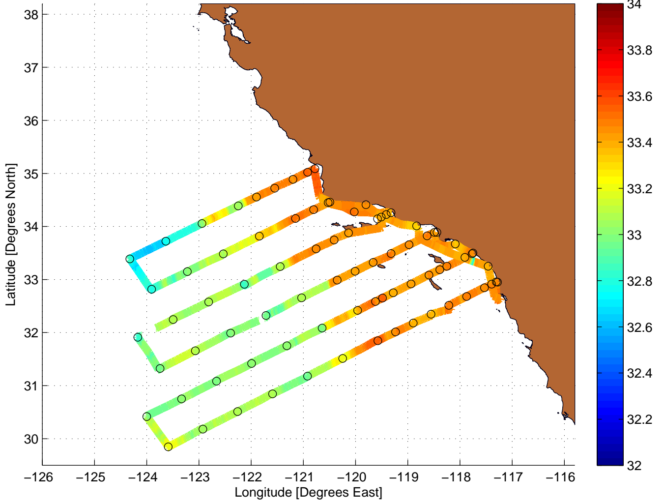
Salinity Value Along CalCOFI Cruise: 0407JD
