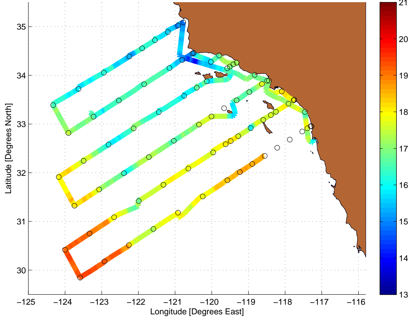
Temperature Value Along CalCOFI Cruise: 0411RR
