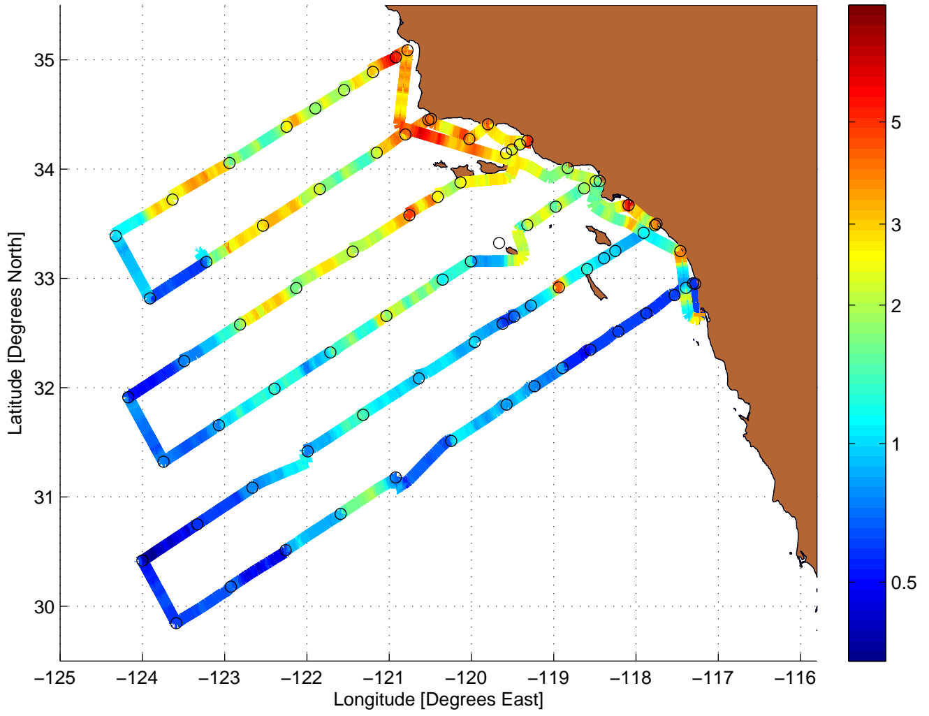
Fluorescence Value Along CalCOFI Cruise: 0411RR
