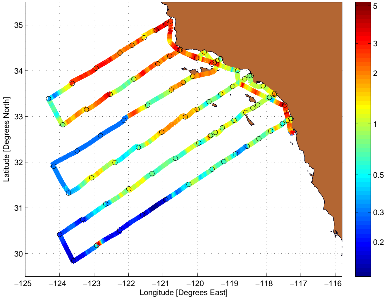
Fluorescence Value Along CalCOFI Cruise: 0501NH
