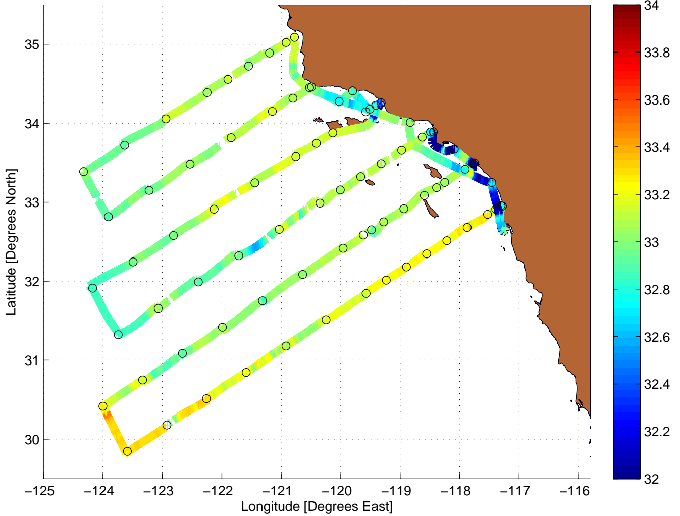
Salinity Value Along CalCOFI Cruise: 0501NH
