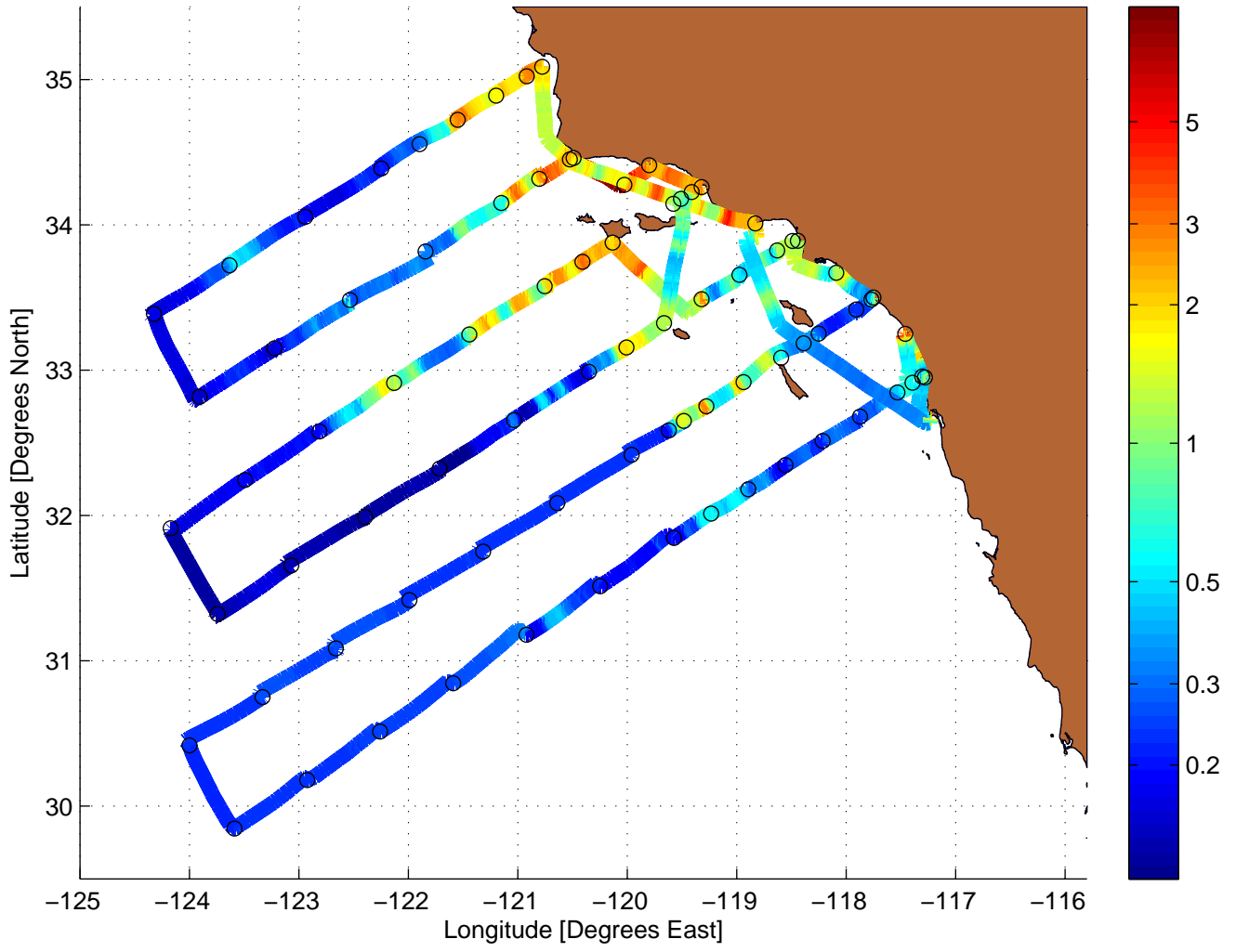
Fluorescence Value Along CalCOFI Cruise: 0504NH
