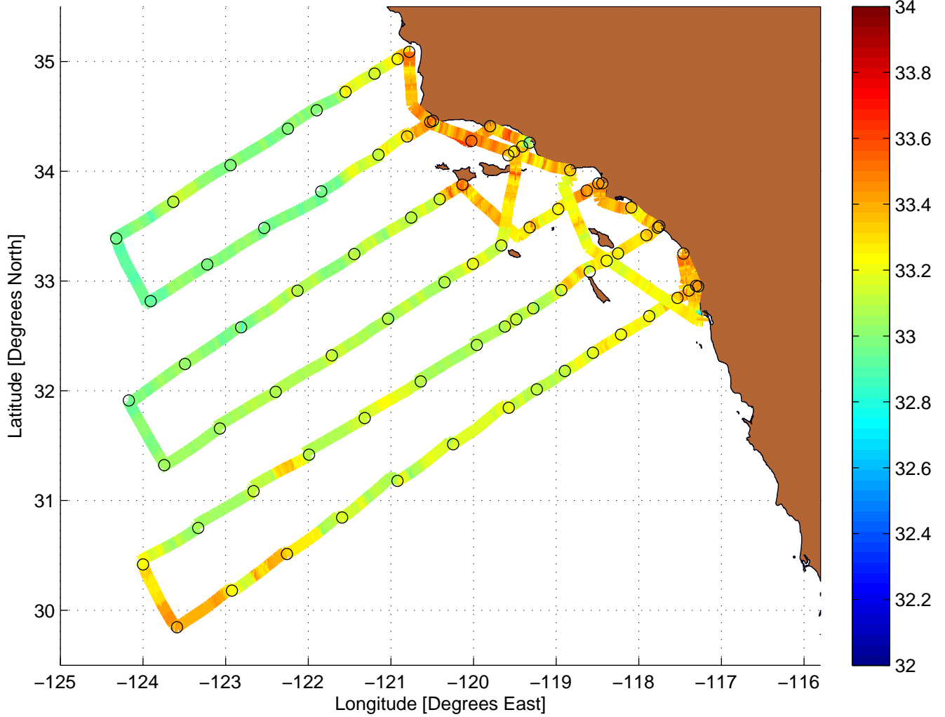
Salinity Value Along CalCOFI Cruise: 0504NH
