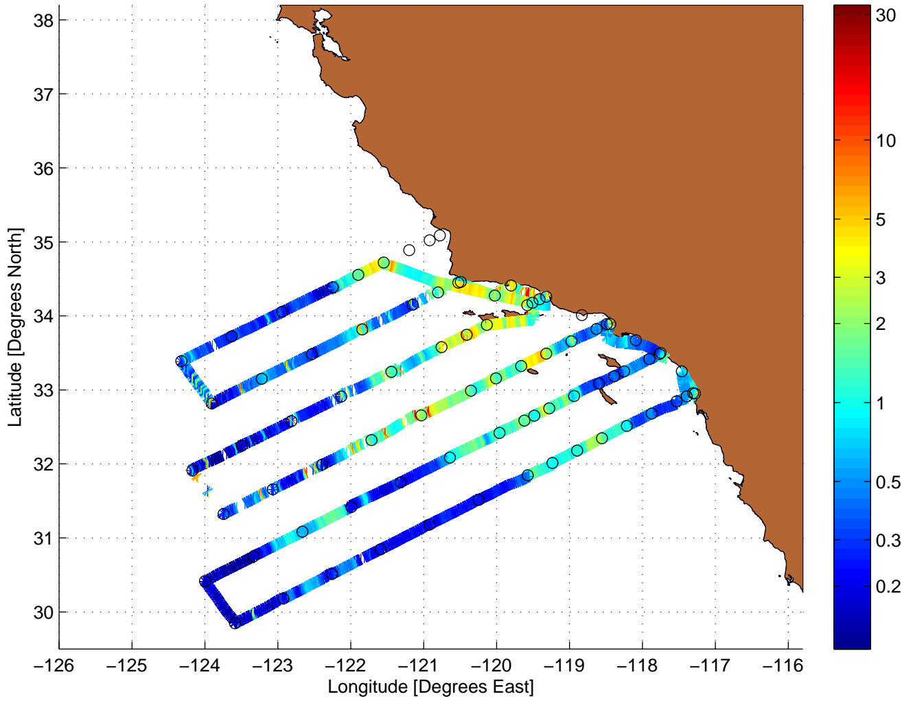
Chlorophylla Value Along CalCOFI Cruise: 0602JD
