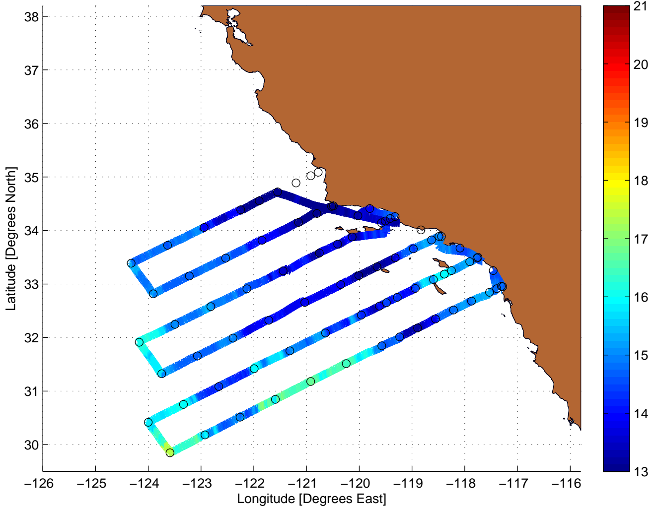
Temperature Value Along CalCOFI Cruise: 0602JD
