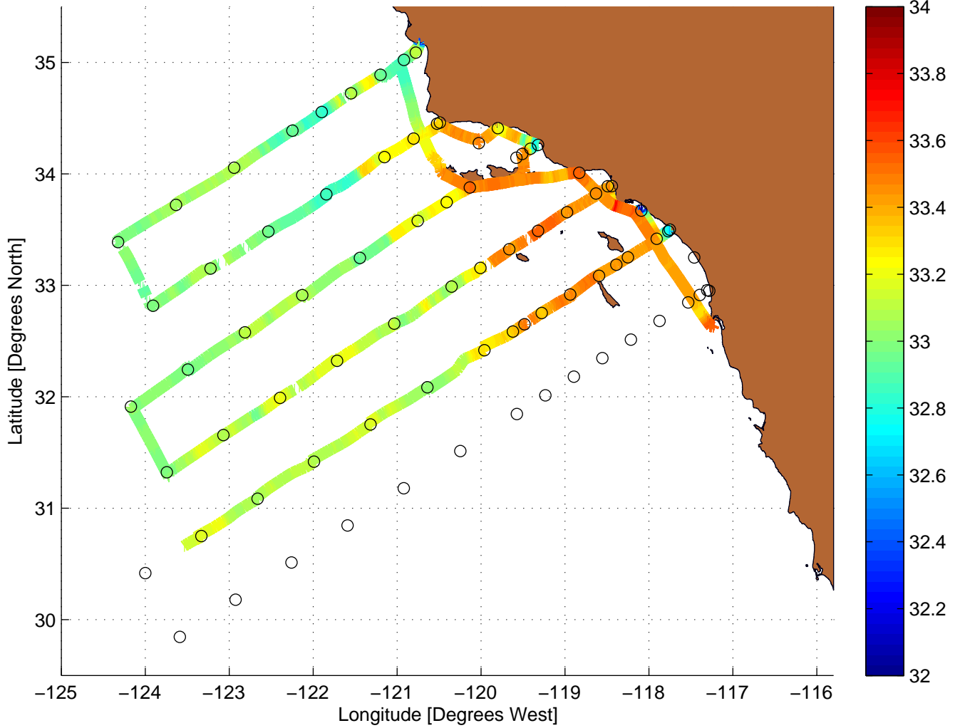
Salinity Value Along CalCOFI Cruise: 0604NH
