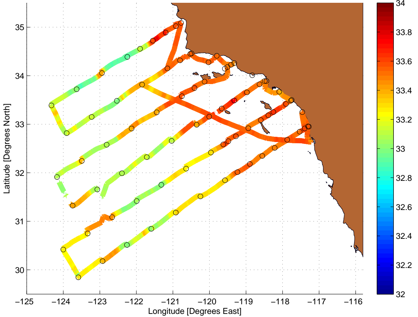
Salinity Value Along CalCOFI Cruise: 0607NH
