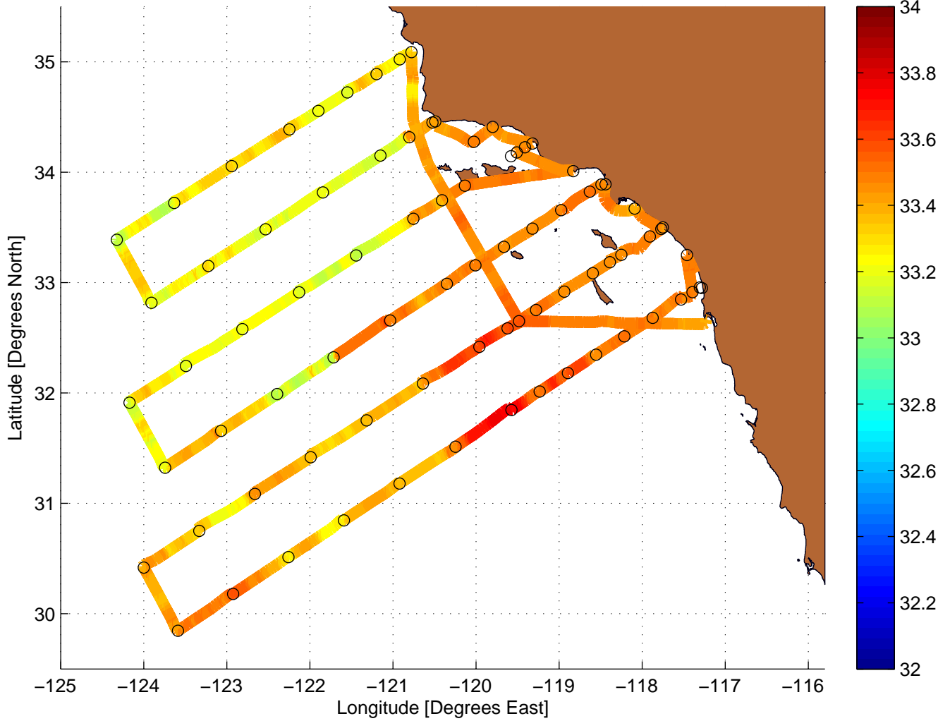
Salinity Value Along CalCOFI Cruise: 0610RR
