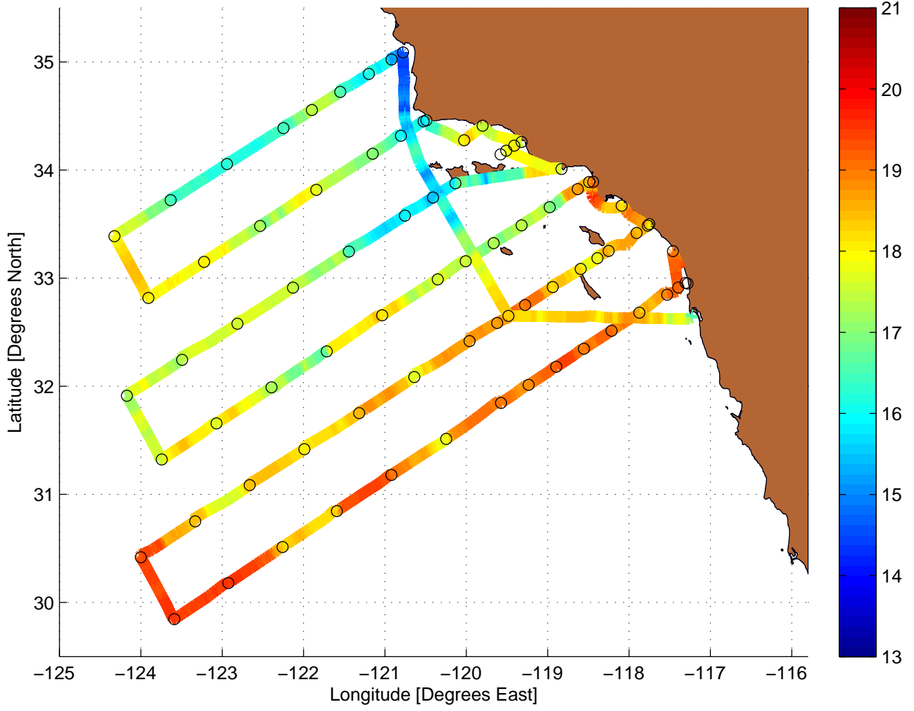
Temperature Value Along CalCOFI Cruise: 0610RR
