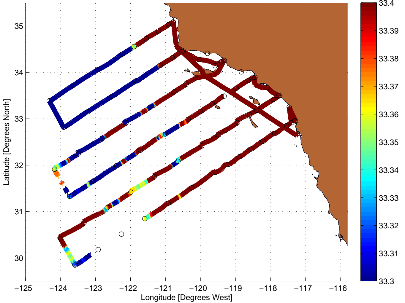
Salinity Value Along CalCOFI Cruise: 0707NH
