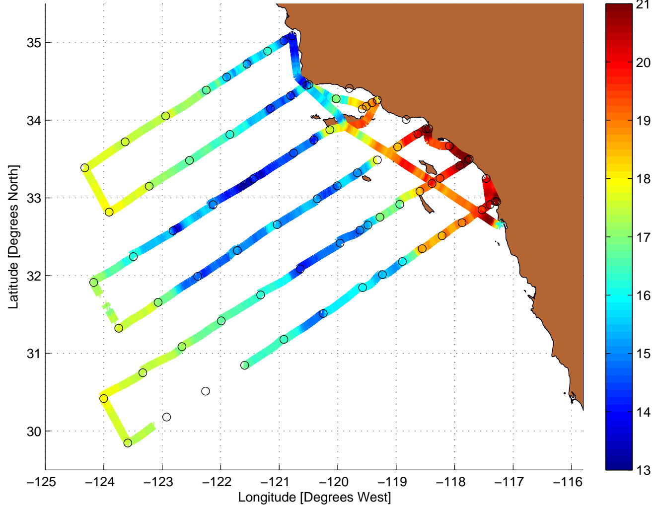
Temperature Value Along CalCOFI Cruise: 0707NH
