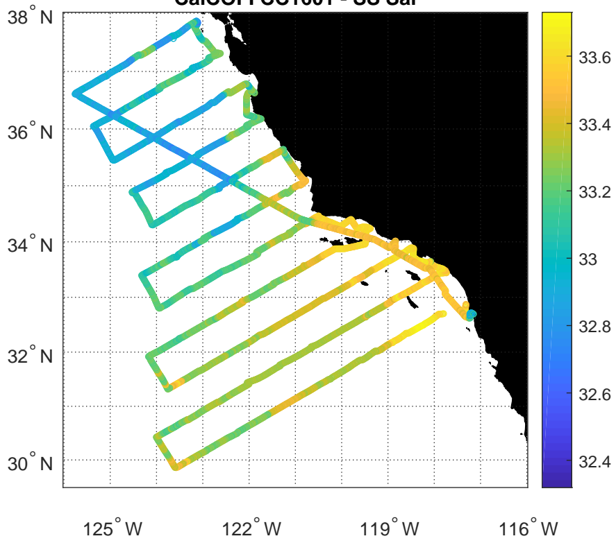
CalCOFI CC1601 - SS Sal
