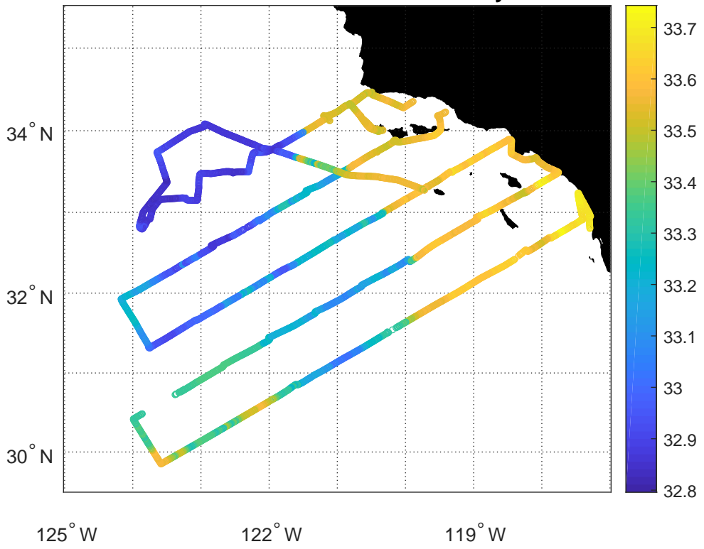
CalCOFI CC1607 - Surface Salinity
