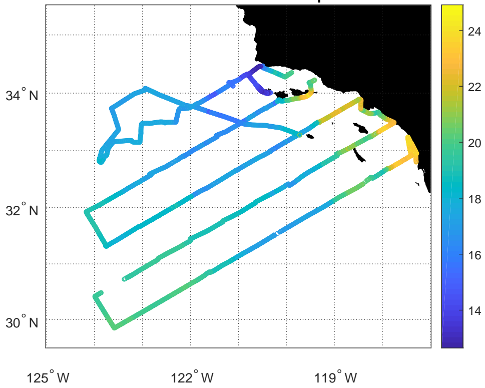
CalCOFI CC1607 - Surface Temperature
