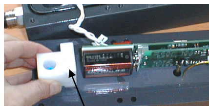
Remove battery cap
