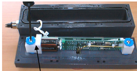
Battery cap - remove Phillips-head screw and grommet
