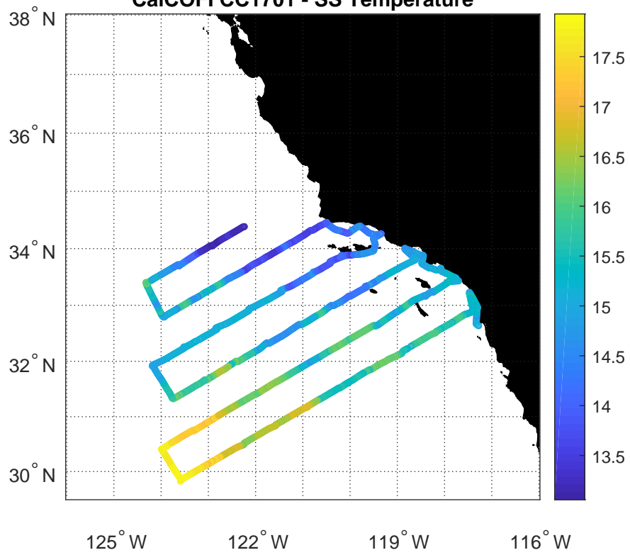
CalCOFI CC1701 - SS Temperature
