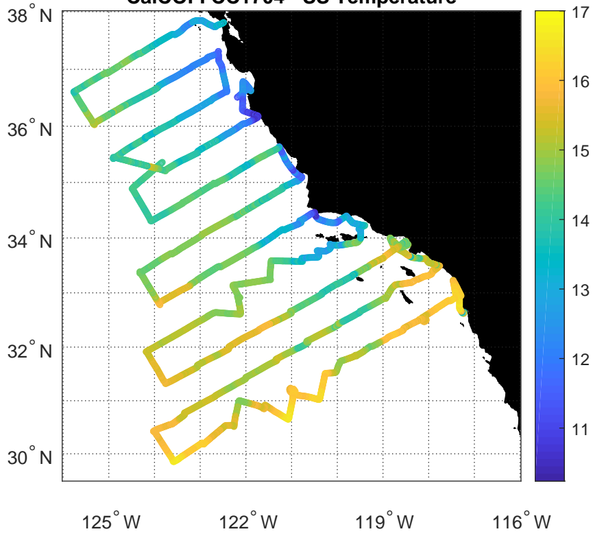
CalCOFI CC1704 - SS Temperature
