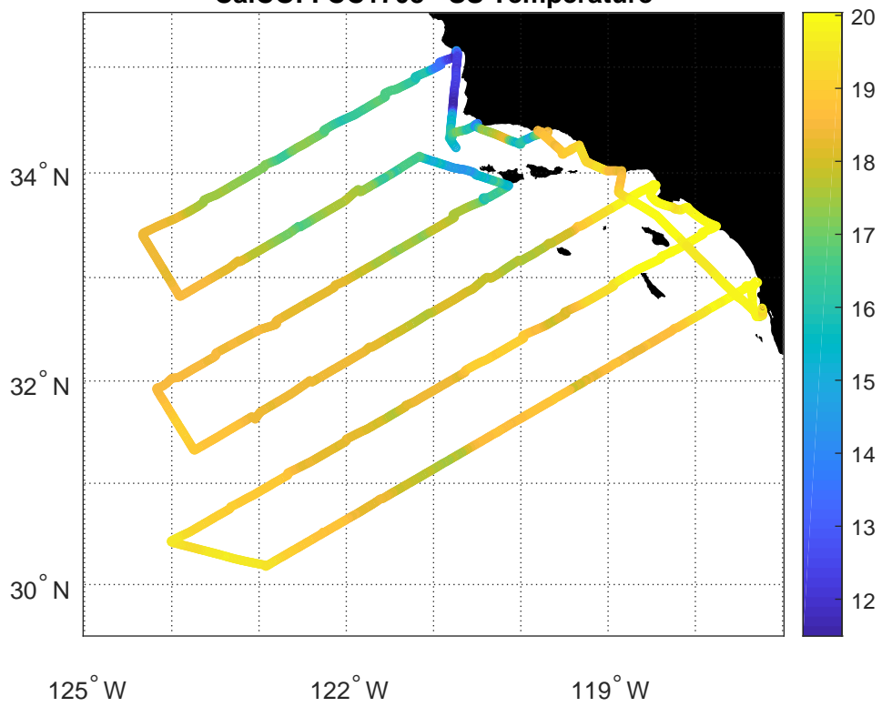
CalCOFI CC1708 - SS Temperature
