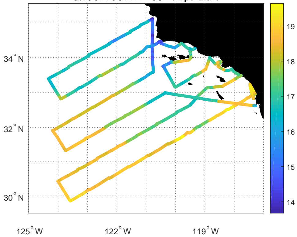
CalCOFI CC1711 - SS Temperature
