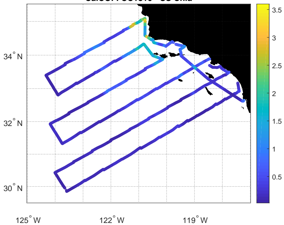
CalCOFI CC1810 - SS Chla
