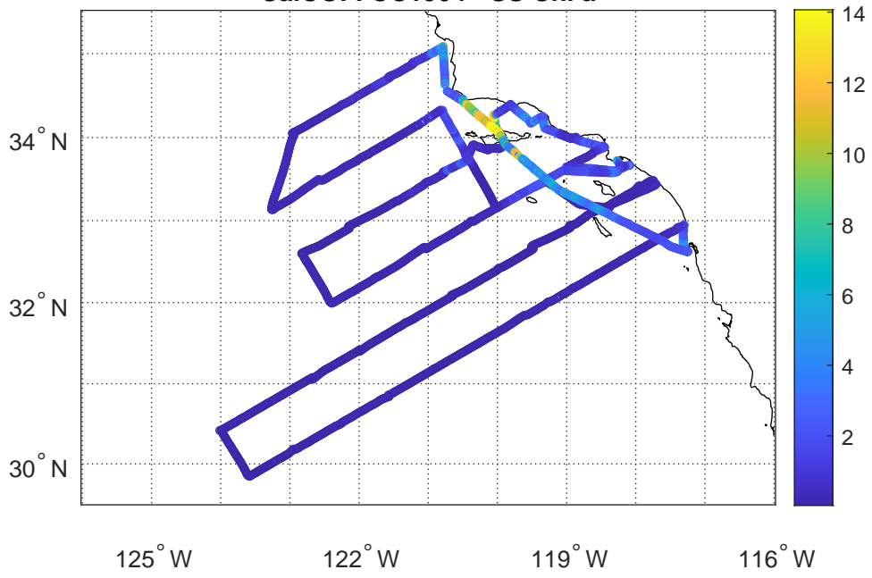
CalCOFI CC1904 - SS Chl a
