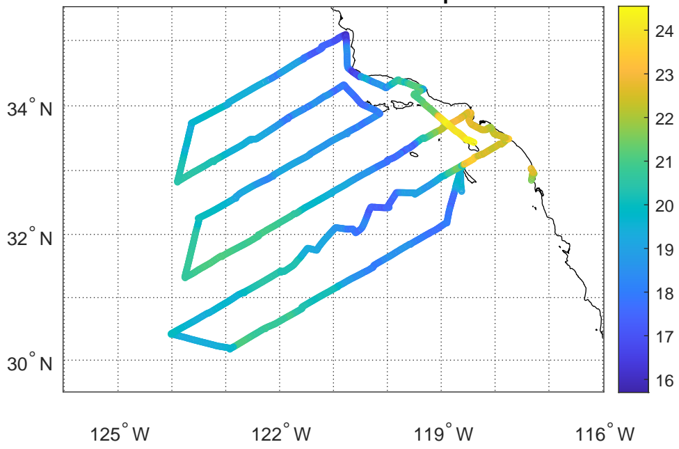
CalCOFI CC1907 - Surface Temperature
