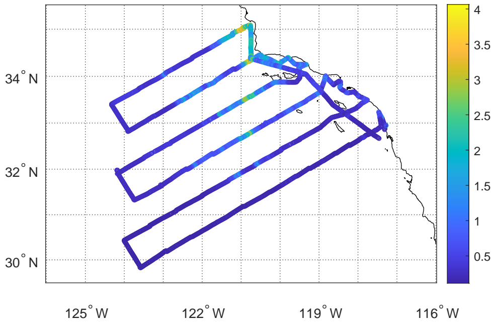
CalCOFI CC1911 - SS Chl a
