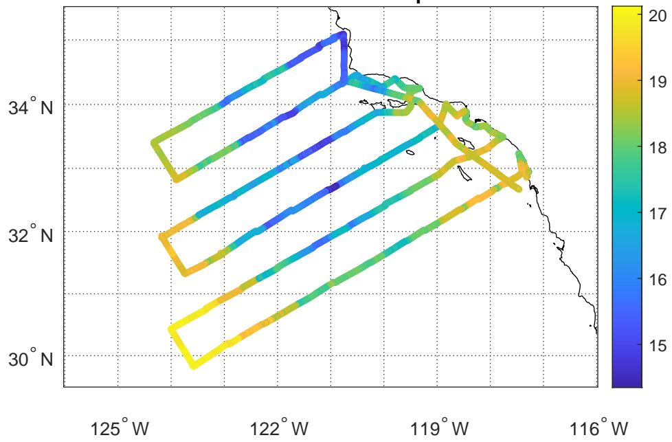
CalCOFI CC1911 - SS Temperature
