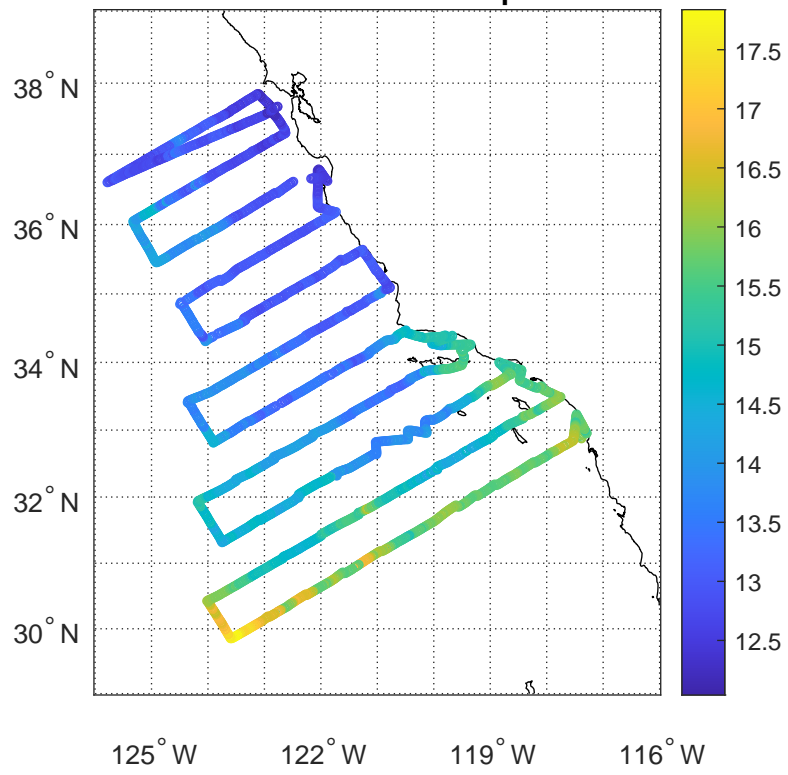
CalCOFI CC2001 - SS Temperature
