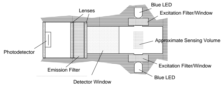
Figure 2. Seapoint Chlorophyll Fluorometer Optics
