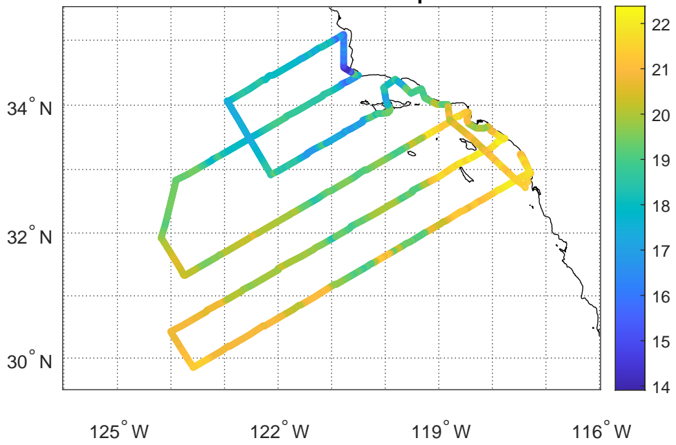
CalCOFI CC2010 - SS Temperature
