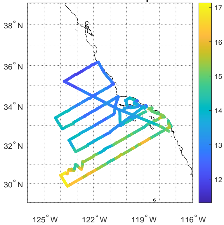
CalCOFI CC2101 - SS Temperature
