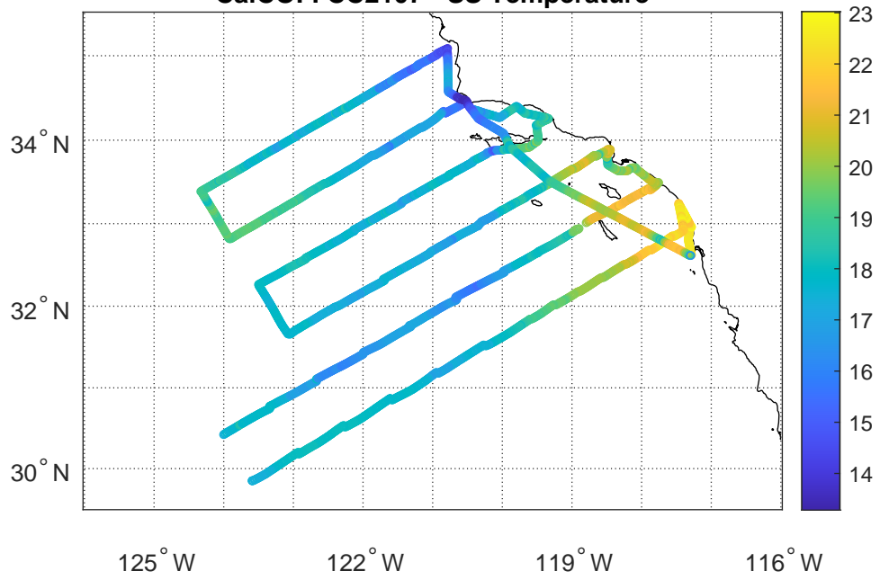
CalCOFI CC2107 - SS Temperature
