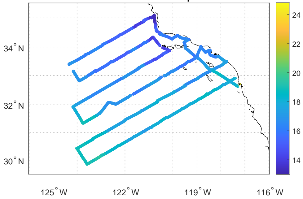
CalCOFI CC2111 - SS Temperature
